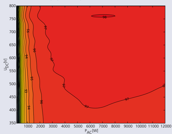
3D-Wirkungsgraddiagramm Powador 14.0 TL3
